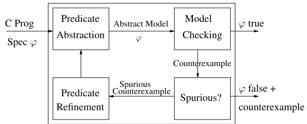
Fig. 2 The CEGAR framework
