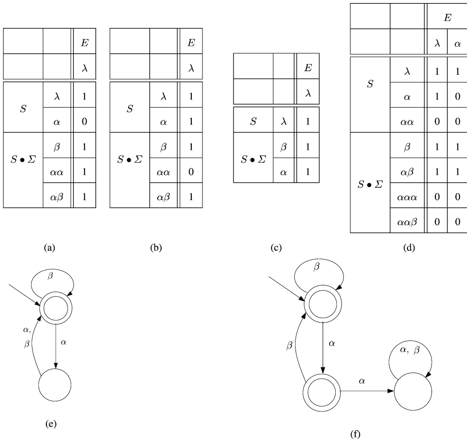
Fig. 8 Illustration of the revalidation procedure described in Example 2; (a) Observation table for original language U = (\beta \mid (\alpha \bullet (\alpha \mid \beta)))^* ; (b) New observation table after recomputing the entries with respect to the new language U' = ((\beta \mid \alpha \bullet \beta)^*) \mid ((\beta \mid \alpha \bullet \beta)^* \bullet \alpha) ; e.g., \alpha \in U' implies T(\alpha, \lambda) = 1 ; (c) Observation table after revalidating with respect to U' and (d) after an L^* learning iteration with respect to U' ; (e) DFA for language U (corresponding to observation table in (a)); and (f) DFA for language U' (corresponding to table in (d))
